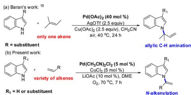
Scheme 1. Pd-Catalyzed Oxidative Cross-Coupling Reactions of Indoles with Alkenes
