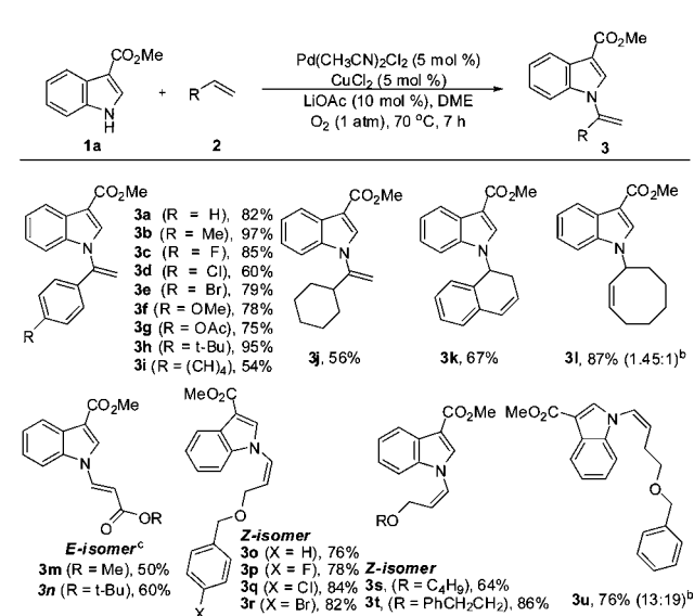
Scheme 2. Scope of Alkenes in the Direct N-Alkenylation of Indole a
