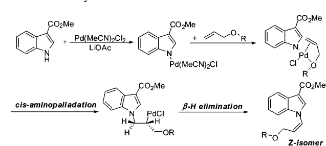
Scheme 3. Possible Reaction Pathway for the N -Alkenylation of Indole with Allylic Ether
