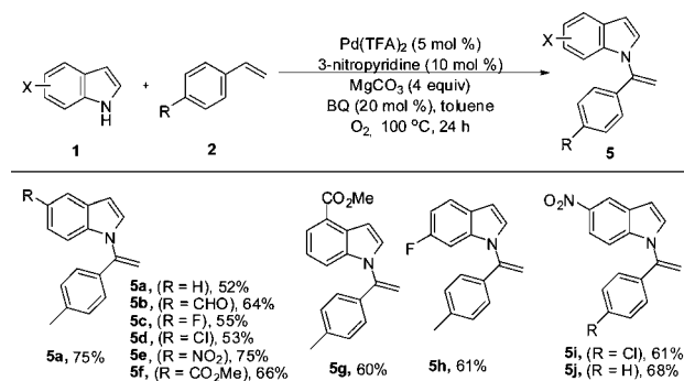
Scheme 5. Scope of Simple Indoles a
