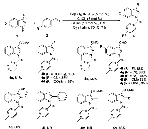
Scheme 4. Scope of 3-Substituted Indoles in the Direct N-Alkenylation of Indole a
